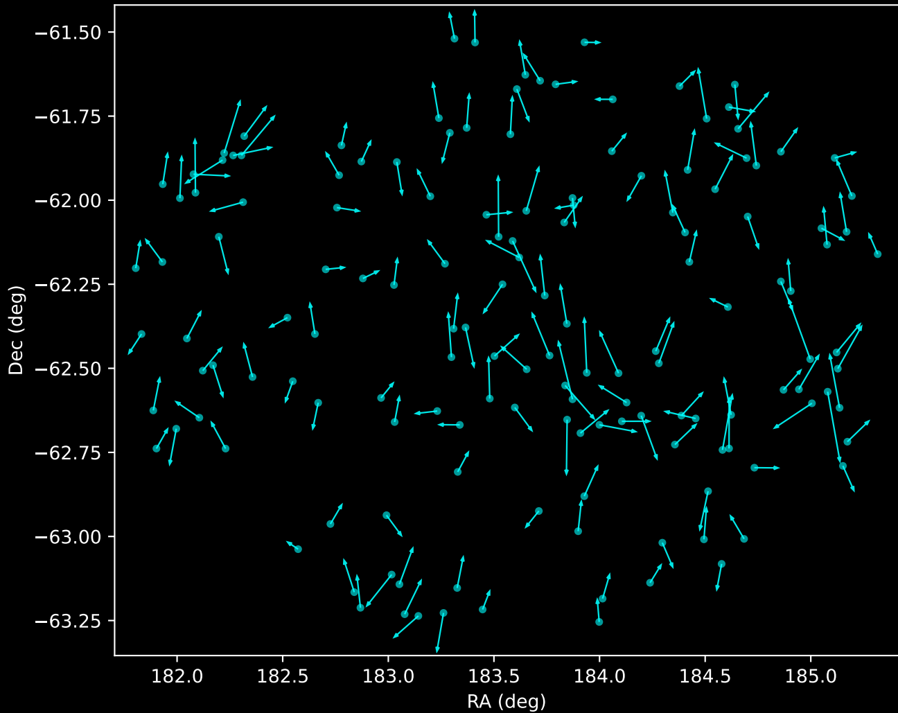
GALAH DR4 Noise Stream Proper Motion Vectors (n=150)
