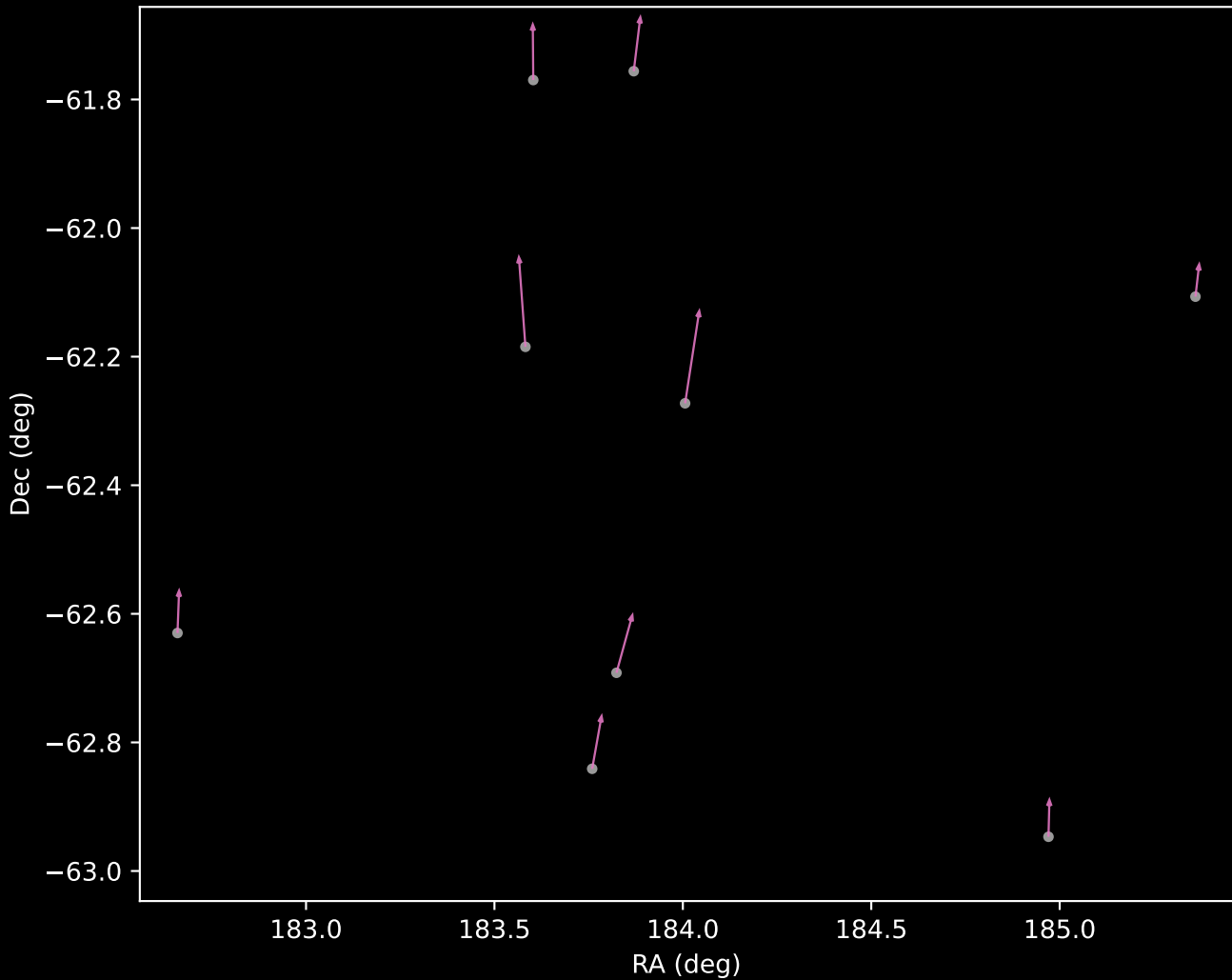
GALAH DR4 Cluster 12 Proper Motion Vectors (n=9)
