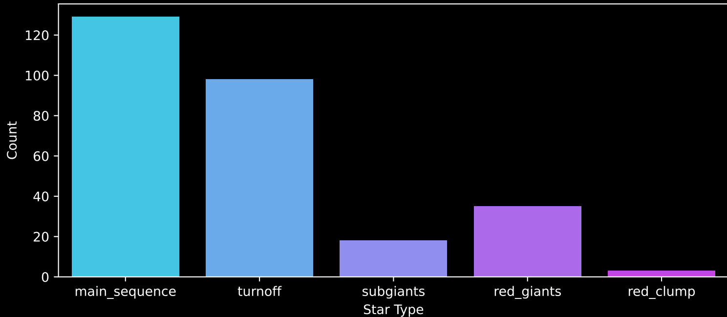
GALAH DR4 Field: [677] Count plot of Star Type
