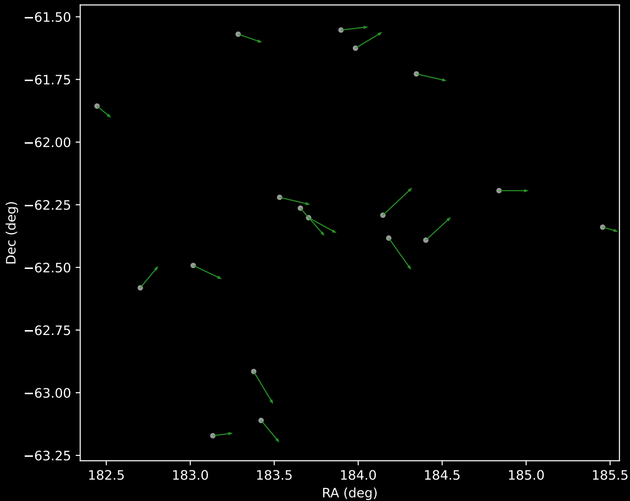
GALAH DR4 Cluster 4 Proper Motion Vectors (n=18)
