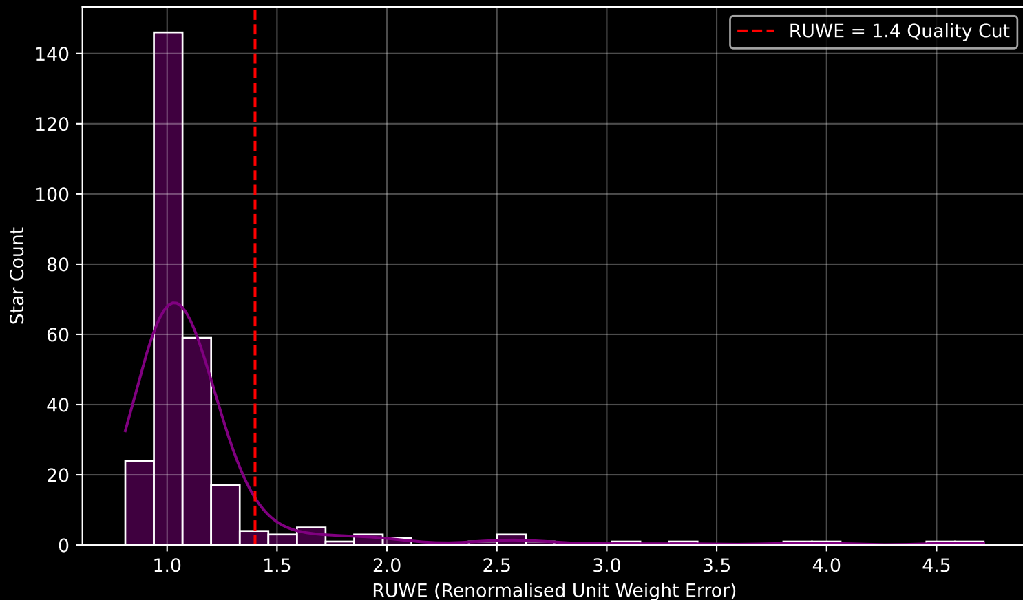
GALAH DR4 Field [677] RUWE Distribution (n= 275)
