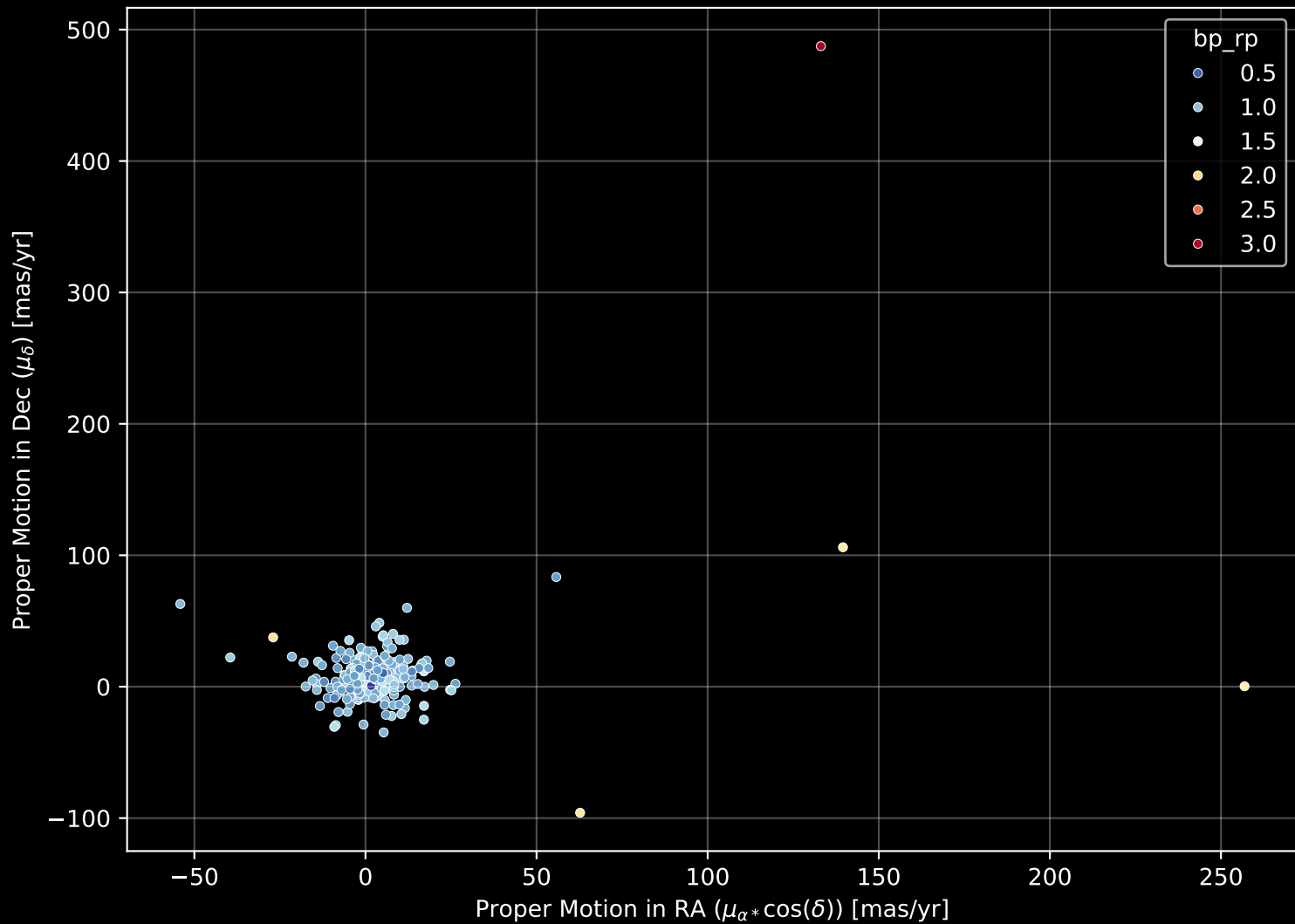
GALAH DR4 Field: [677] Proper Motion Diagram (n= 283)
