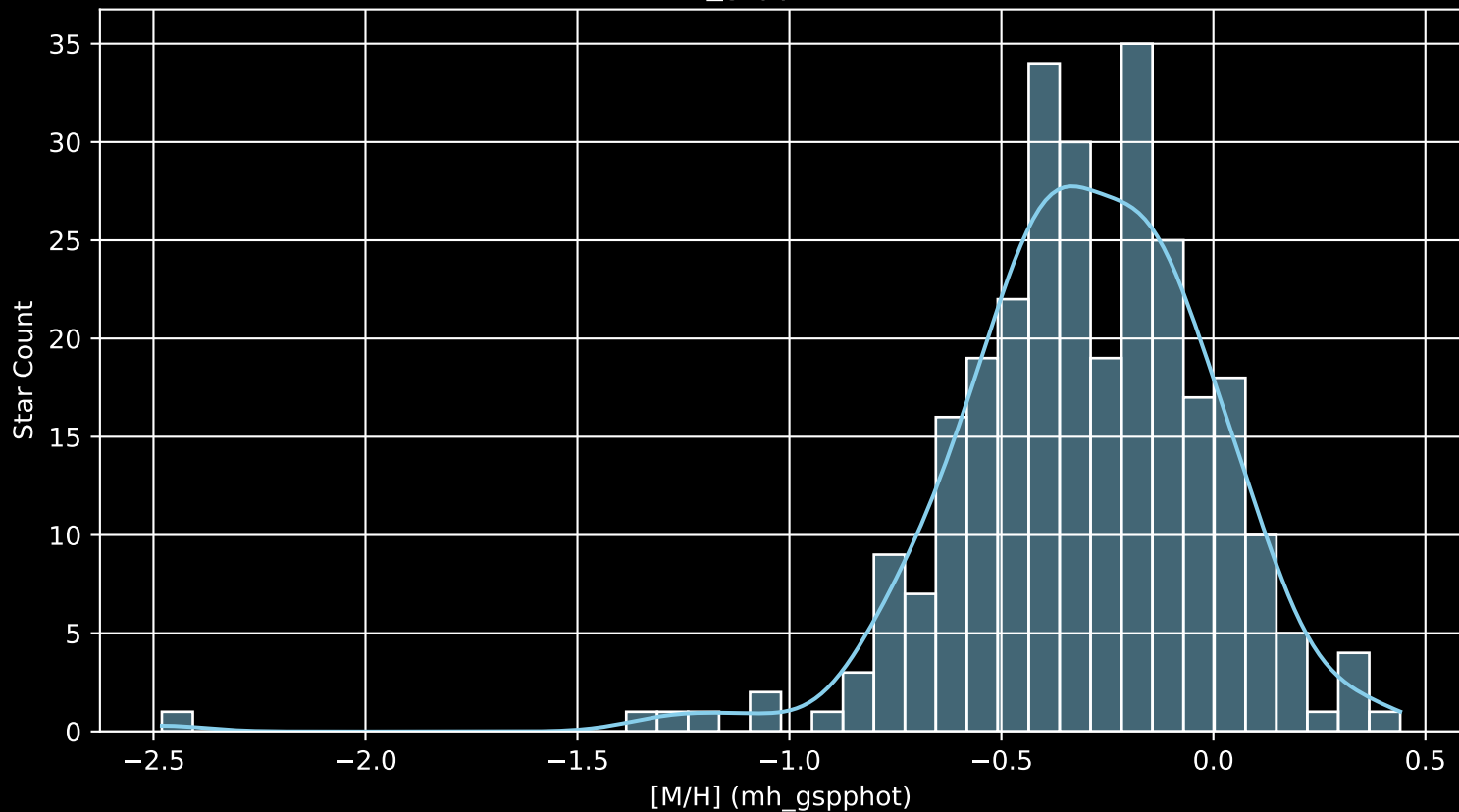
GALAH DR4 Field: [677] [M/H] (mh_gspphot) (n= 282)
