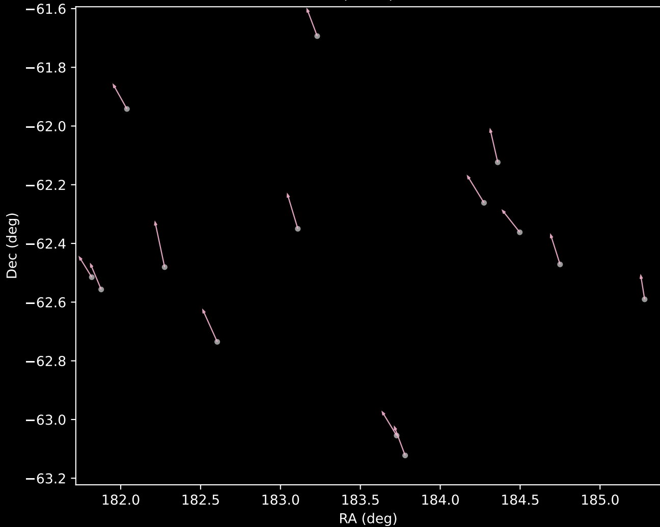
GALAH DR4 Cluster 13 Proper Motion Vectors (n=14)
